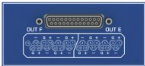
REAR PAN1x DB-25 ("TASCAM")
