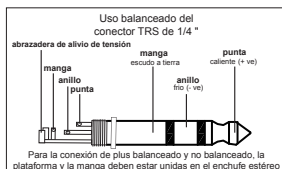
Fig. 8.4: conector 1/4 " TRS
