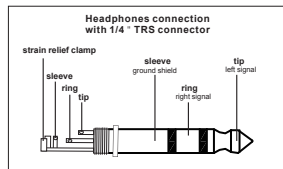
Fig. 8.5: 1/4" TRS connector for headphones
