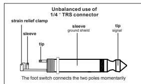
Fig. 8.3: 1/4" TRS connector
