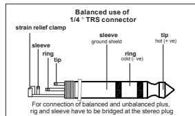
Fig. 8.4: 1/4" TRS connector
