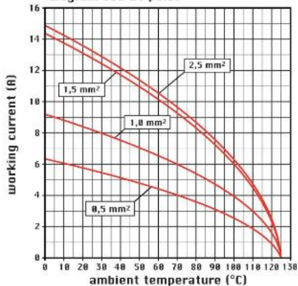
diagram CDD 24 poles
